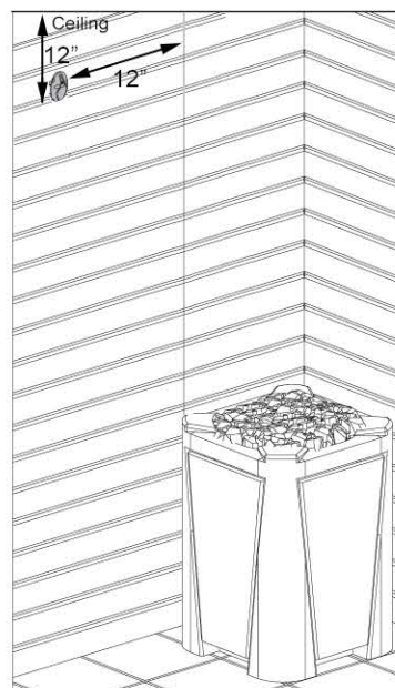
Figure 10. Sensor distance from side of heater
