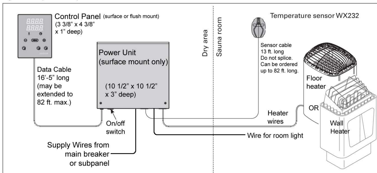
Figure 1. System components
