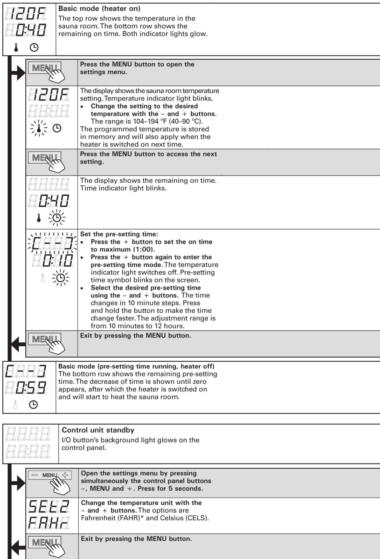
Figure 3. Settings menu structure
