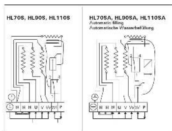
Electrical connections
